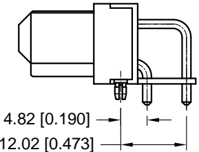
SIZE 16 CONTACTS
