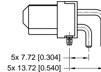
SIZE 12 CONTACTS
