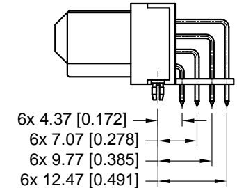
SIZE 22 CONTACTS
